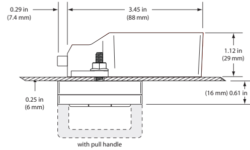
Screw Post 0.01-0.480 in (0.0-12.2 mm) door thickness
