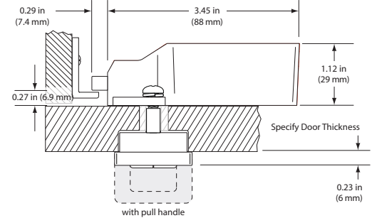
Nut Post 0.850-2.368 in (21.6-60.1 mm) door thickness
