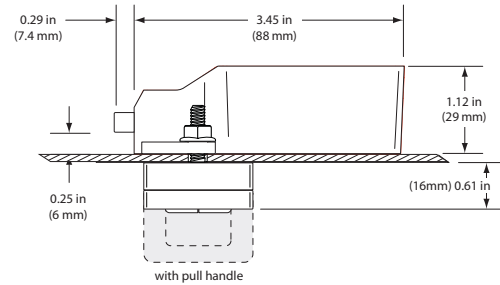
Screw Post 0.01-0.480 in (0.0-12.2 mm) door thickness
