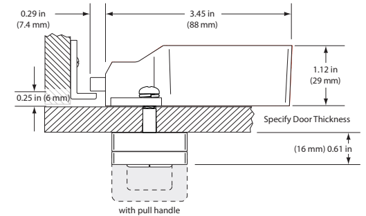
Nut Post 0.480-1.998 in (12.2-50.7 mm) door thickness
