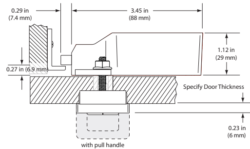
Screw Post 0.370-0.850 in (9.4-21.6 mm) door thickness
